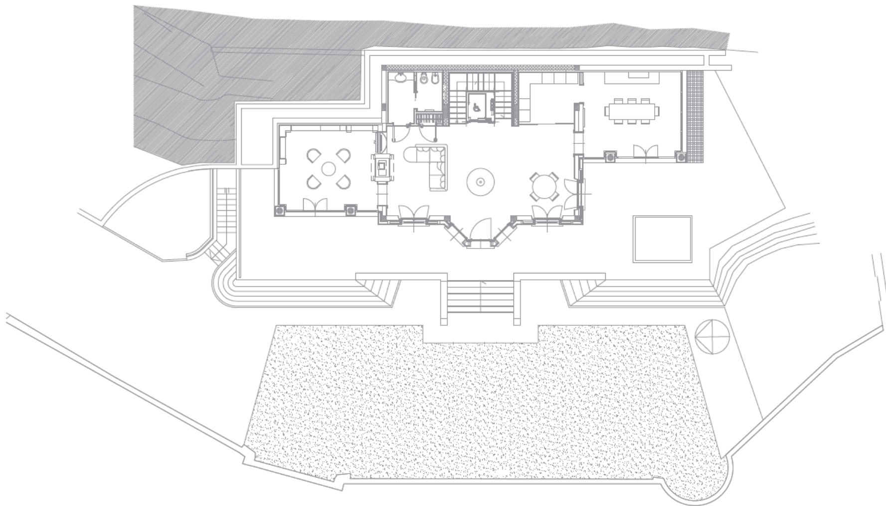
Villa del Lago – Ground Floor
